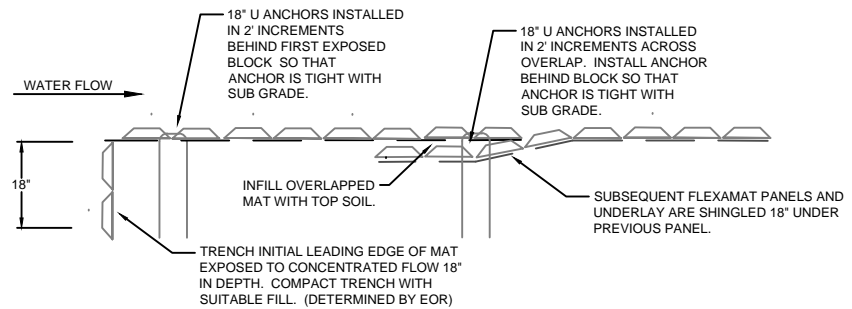
PROFILE VIEW PERPENDICULAR OVERLAPS
